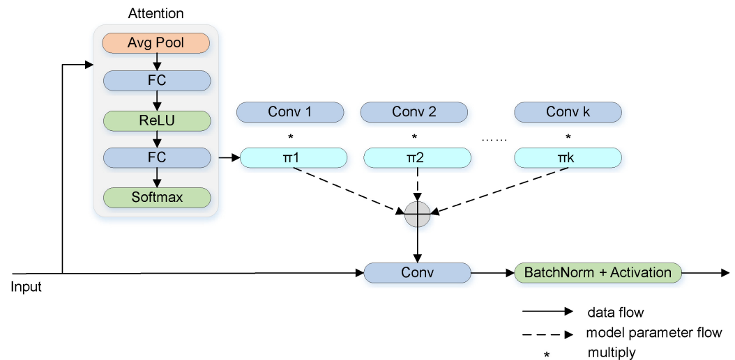
Figure 3. Dynamic convolution [37].
