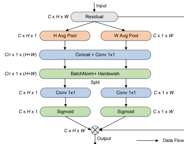
Figure 1. Coordinate attention [29].
