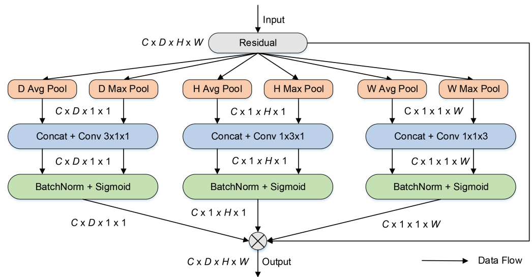
Figure 2. Improved coordinate attention.
