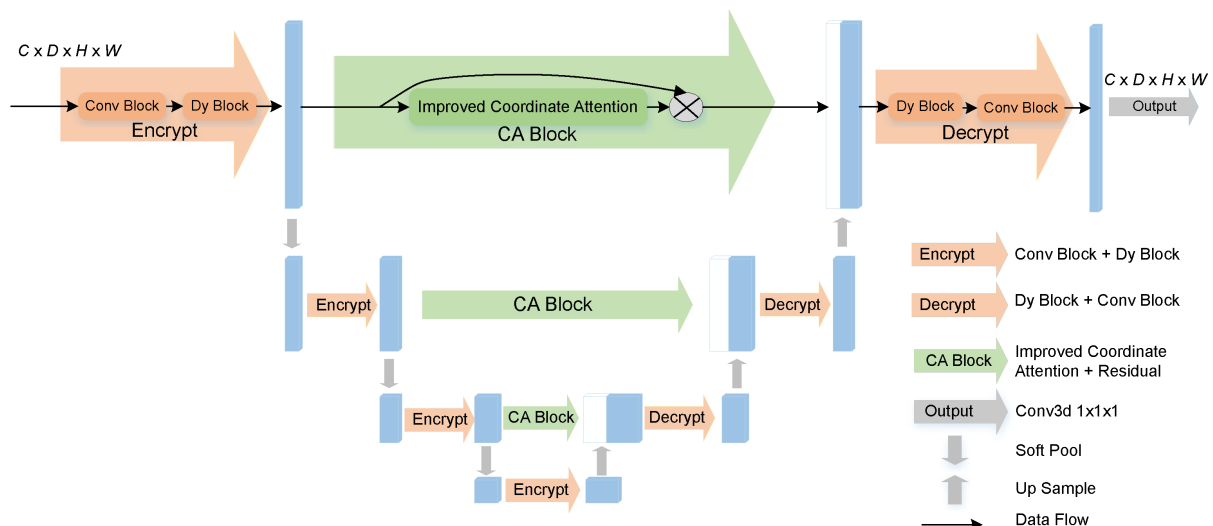
Figure 5. The proposed CADyUNet.
