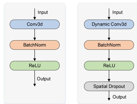
Figure 4. Conv-block and dy-block.
